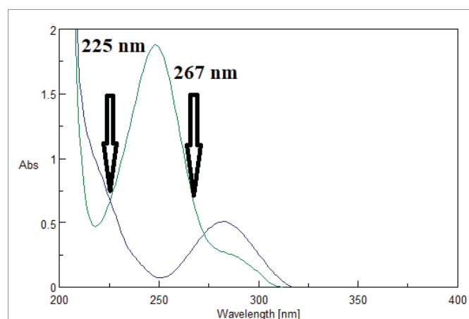
Figure 2: Zero absorption spectrum of 20 \mu\text{g/mL} DCL (blue line) overlaid with 20 \mu\text{g/mL} PAR (green line) revealed that 225 and 267 nm has the same absorbance for PAR spectrum.
