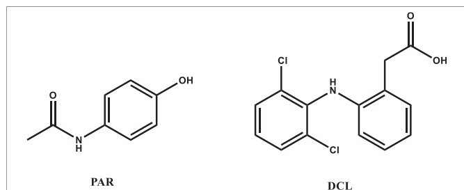
Figure 1: Chemical structures of paracetamol (PAR) and diclofenac (DCL).
