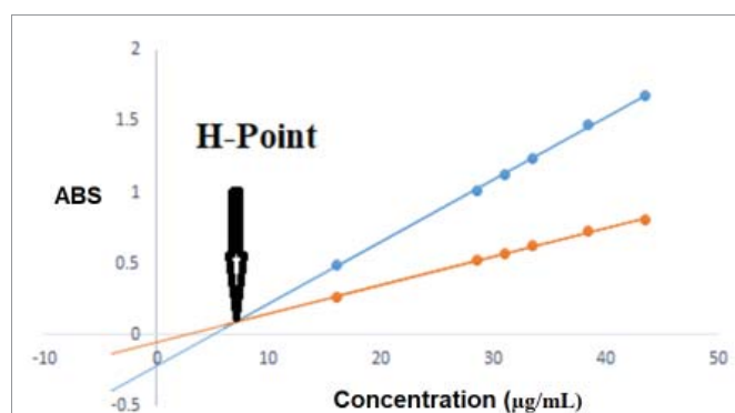
Figure 4: H-Point in the intercept of the two straight lines at 225nm & 267 nm after standard addition of DCL.
