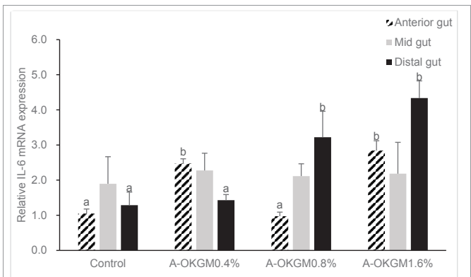
Figure 5: Effects of A-OKGM on IL-6 expression in anterior, mid and distal gut of Schizothorax prenanti . The observed values were expressed as mean ± S.E. Mean values with different superscripts are significantly ( P < 0.05 ) different from each other.
