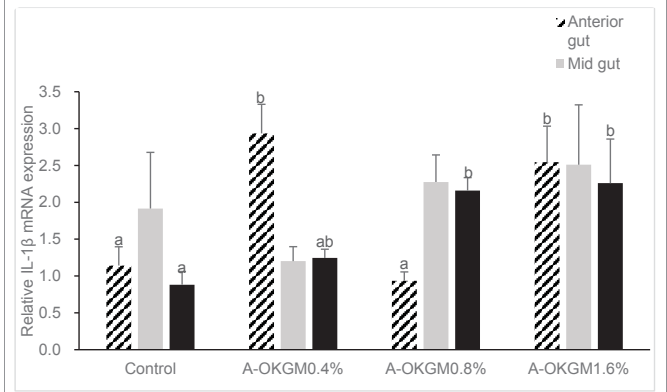
Figure 4: Effects of A-OKGM on IL-1β expression in anterior, mid and distal gut of Schizothorax prenanti . The observed values were expressed as mean ± S.E. Mean values with different superscripts are significantly ( P < 0.05 ) different from each other.
